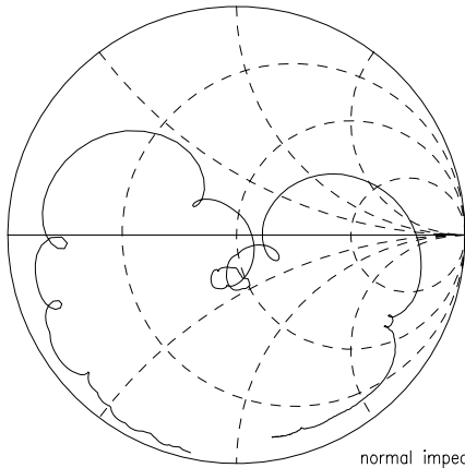
normal impedance: 50.00 \Omega
