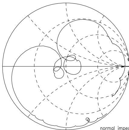
normal impedance: 150.0 \Omega
